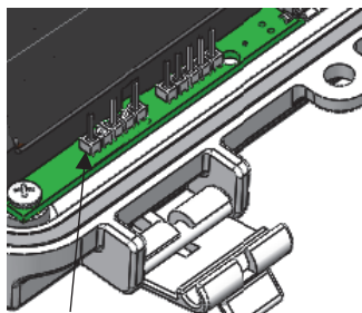
Connect the programming tool to these connection pins
